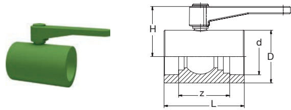
BR PP-R Kugelhahn grün BR PP-R Ball valve green
