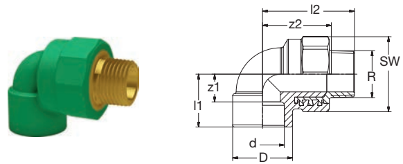
BR PP-RCT-RG/LFB Ü-Winkel 90° AG-keg grün BR PP-RCT-Bronze/LFB Transition-Elbow 90° male-thread-con green
