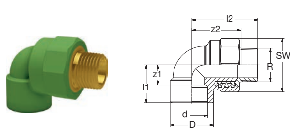
BR PP-R-LFB Ü-Winkel 90° AG-keg grün
