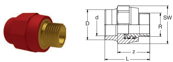
BR PP-CFR- Ms/LFB Übergang AG-keg rot
