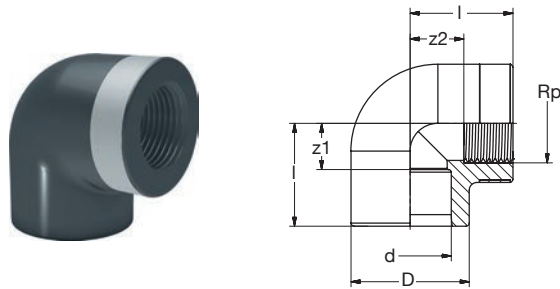
BR PVC-U Ü-Winkel 90° IG-zyl grau
