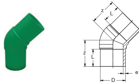
BR PP-RCT Winkel 45° lang st grün BR PP-RCT Elbow 45° long butt green
