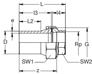
BR PE100- V2A Ü-Verschraubung lang IG-zyf Flachdichtring-EPDM SDR11 schwarz BR PE100- Stainless steel Transition-Union long female-thread-cyl SDR11 black
