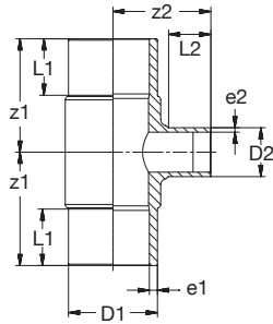
BR PE100 T-Stück 90° red lang SDR11 schwarz BR PE100 Tee 90° red long SDR11 black
