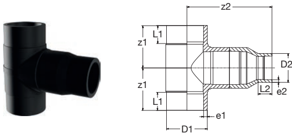
BR PE100 T-Stück 90° red lang Form-B SDR11 schwarz BR PE100 Tee 90° red long style-B SDR11 black
